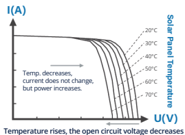
Figure 1-4 Relationship between solar panel output characteristics and temp.
